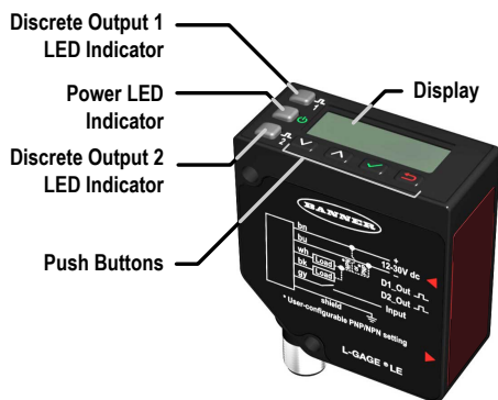
Figure 1. LE IO-Link Sensor Features
