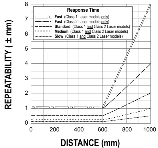
Figure 16. Repeatability (90% to 6% reflectance)
