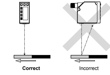
Figure 8. Orientation for a color or luster difference
